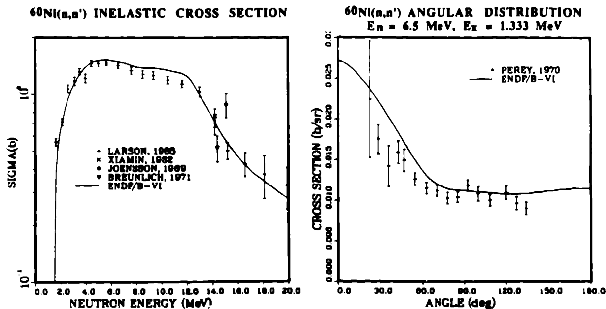
Fig. 4. Calculated and measured data for ^{60}\text{Ni}(n,n') reactions. The solid curves were calculated with the TNG code, 14 and the points represent experimental data. 12 The energy dependence of the ^{60}\text{Ni} total inelastic cross section is shown on the left side; the neutron angular distribution from the ^{60}\text{Ni}(n,n') reaction to the 1.333-MeV state in ^{60}\text{Ni} with 6.5 MeV incident neutrons is shown on the right side of the figure.
